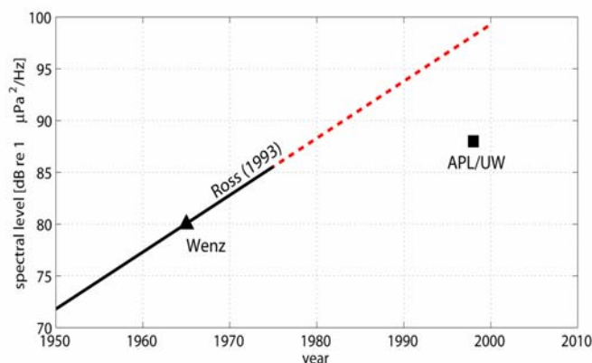
Figure 2: Ambient noise measurements in the 100-200 hertz (Hz) band measured off California in the 1950s (Wenz, 1962; Ross, 1993) and Applied Physics Laboratory/University of Washington (APL/UW) noise measurements in the late 1990s (Andrew et al. , 2002)
