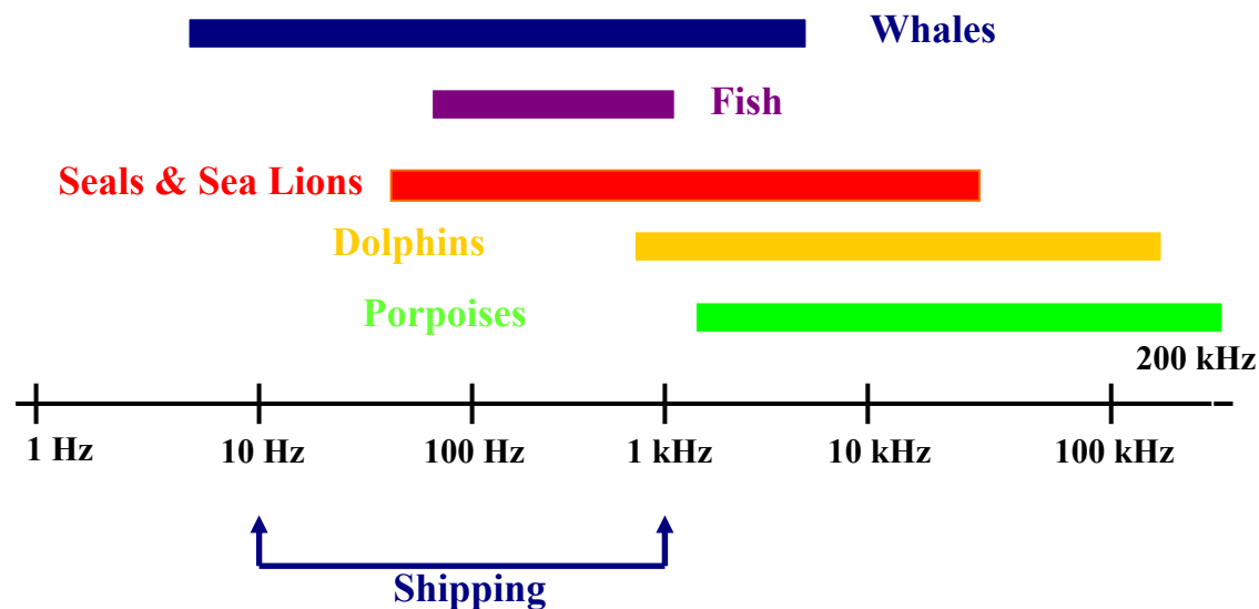
Figure 1: Frequency relationships between marine animal sounds and incidental noise from commercial shipping
